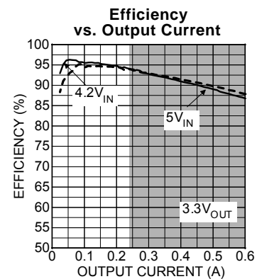
Figure 2. Efficiency Curve
